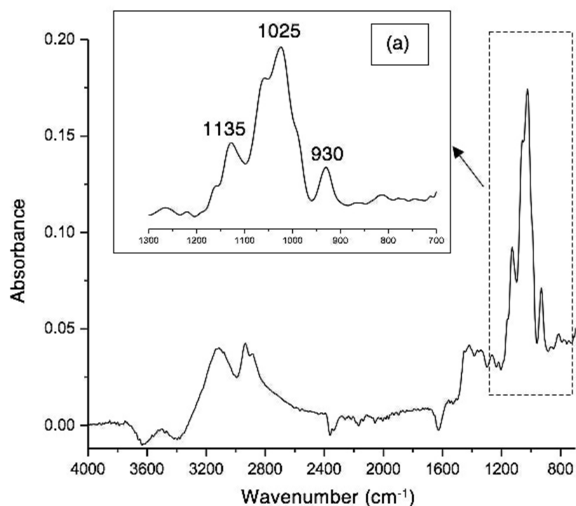
Figure 1. Infrared spectrum of uncooked agave juice. The expanded region ( 1300\text{--}700\text{ cm}^{-1} ) shows the most representative area related to agave fructans.
