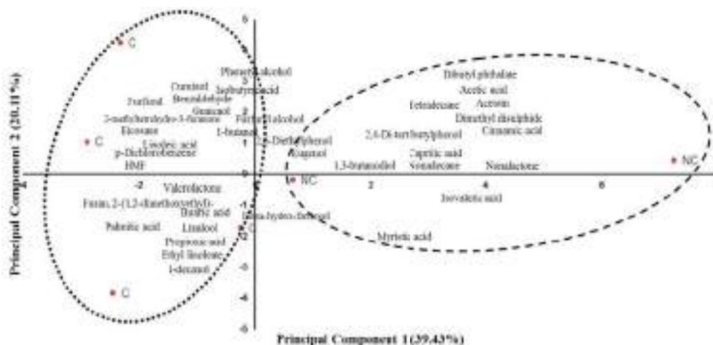
Figure 1. Volatile compounds principal component analysis (PCA) for scores (●) and loadings in tequila vinasses extracts by hydrolysis process.
